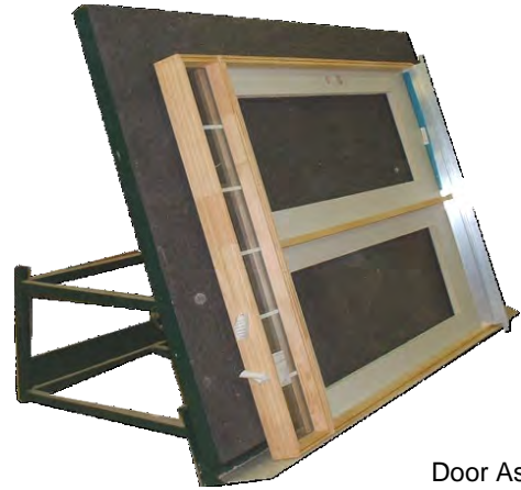
K-29PP Pneumatic Press Patio Door Sash
