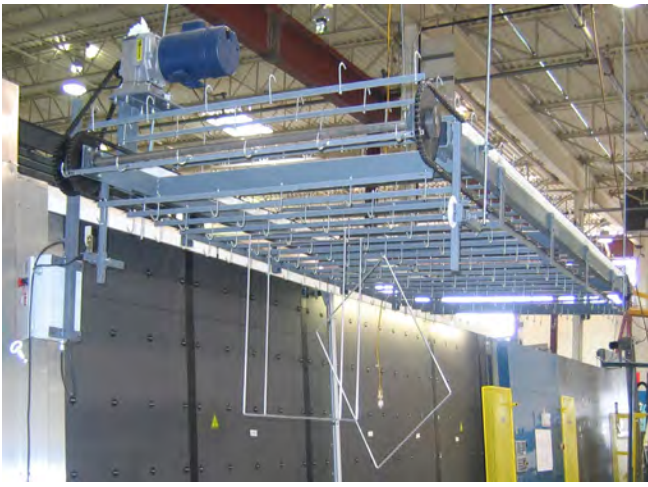
K-53 Overhead Spacer Conveyor
