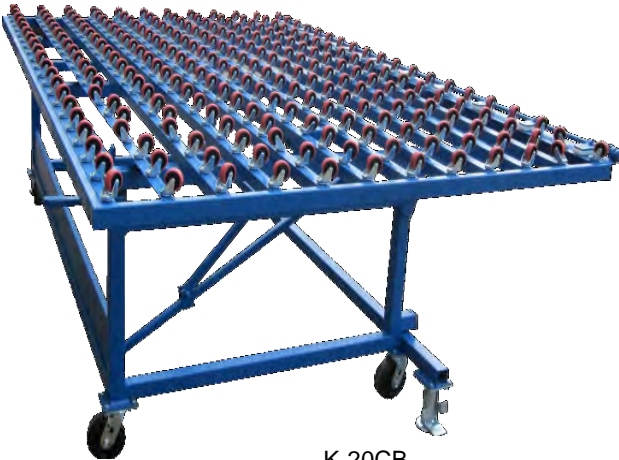
K-20CB Counter -Balance Transfer Table
