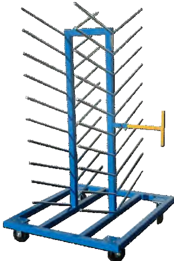
K-27BP Window Frame Dolly
