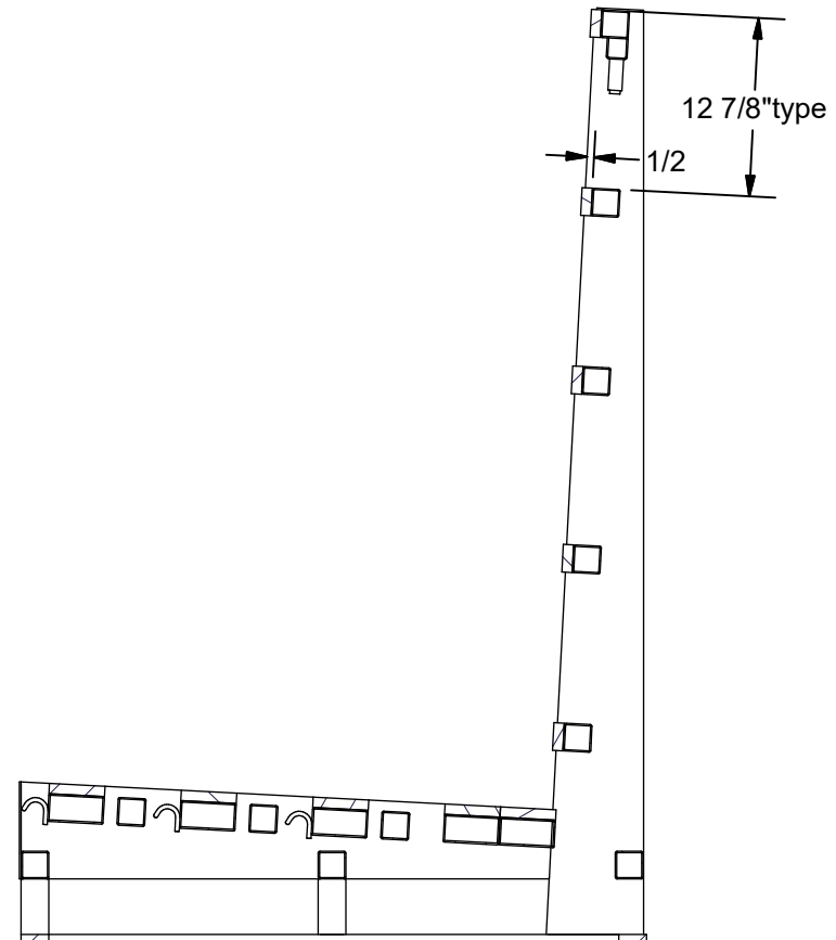
SECTION J-J SCALE 1/15
