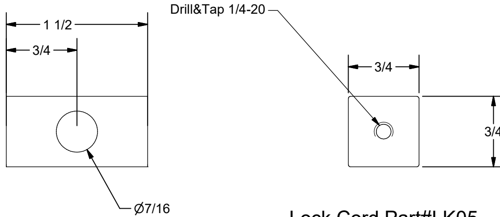
Lock Cord Part#LK05 Material: 3/4" x 3/4" UHMW Square bar Require: 600pcs
